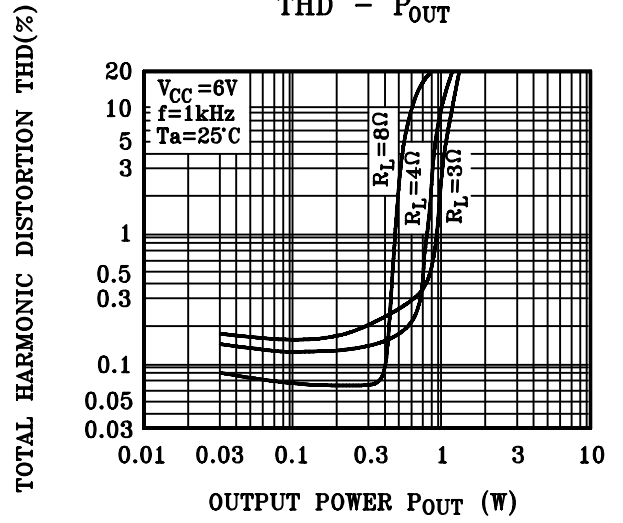
THD - P_{OUT}
